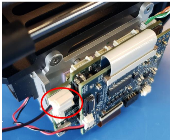
Figure 2: Power Connection
