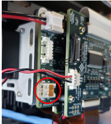
Figure 5: HDMI Connection
