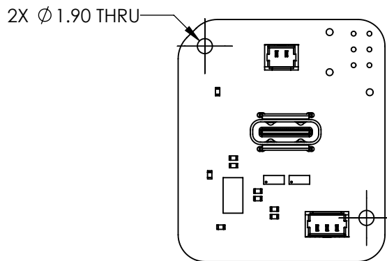
PCBA, DRS USBC Adapter APPROX MASS 3g
