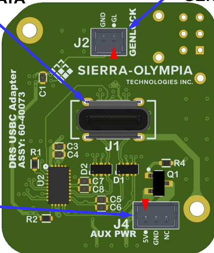
Board Top
